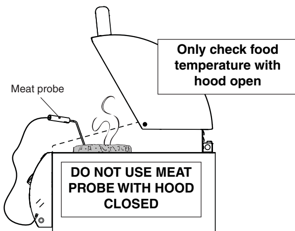
Fig. 26-3 Meat probe
