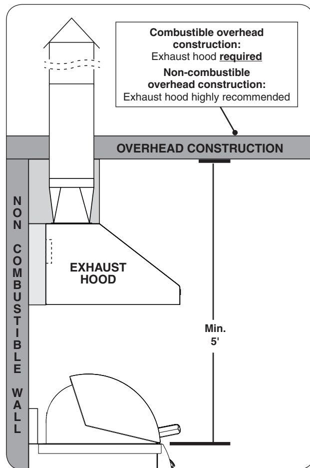
Fig. 11-1 Overhead requirements
