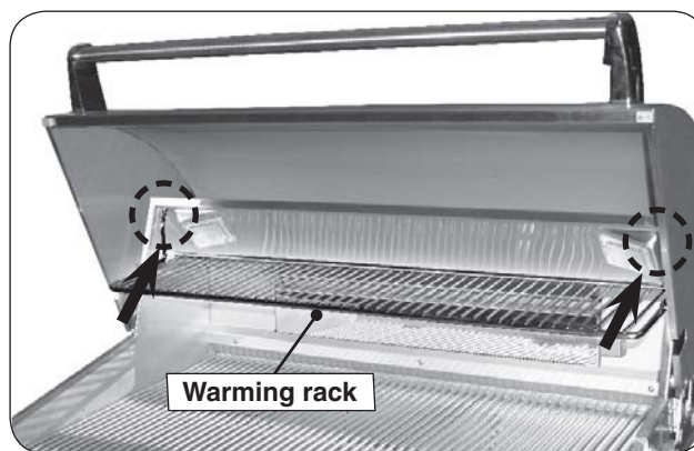
Fig. 20-2 Install warming rack
