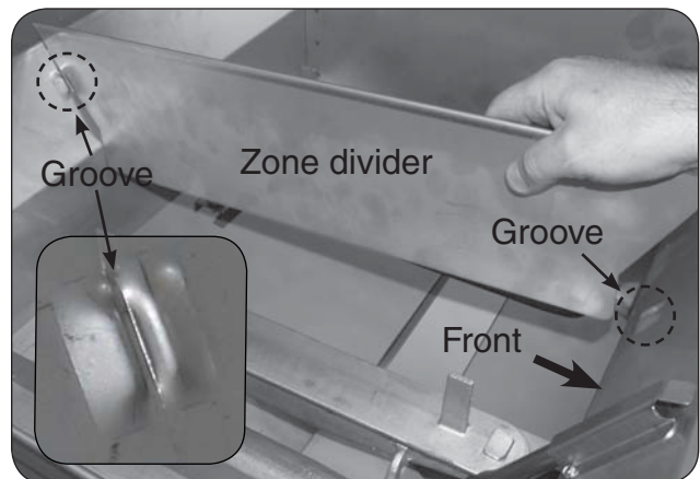
Fig. 19-2 Install zone dividers
