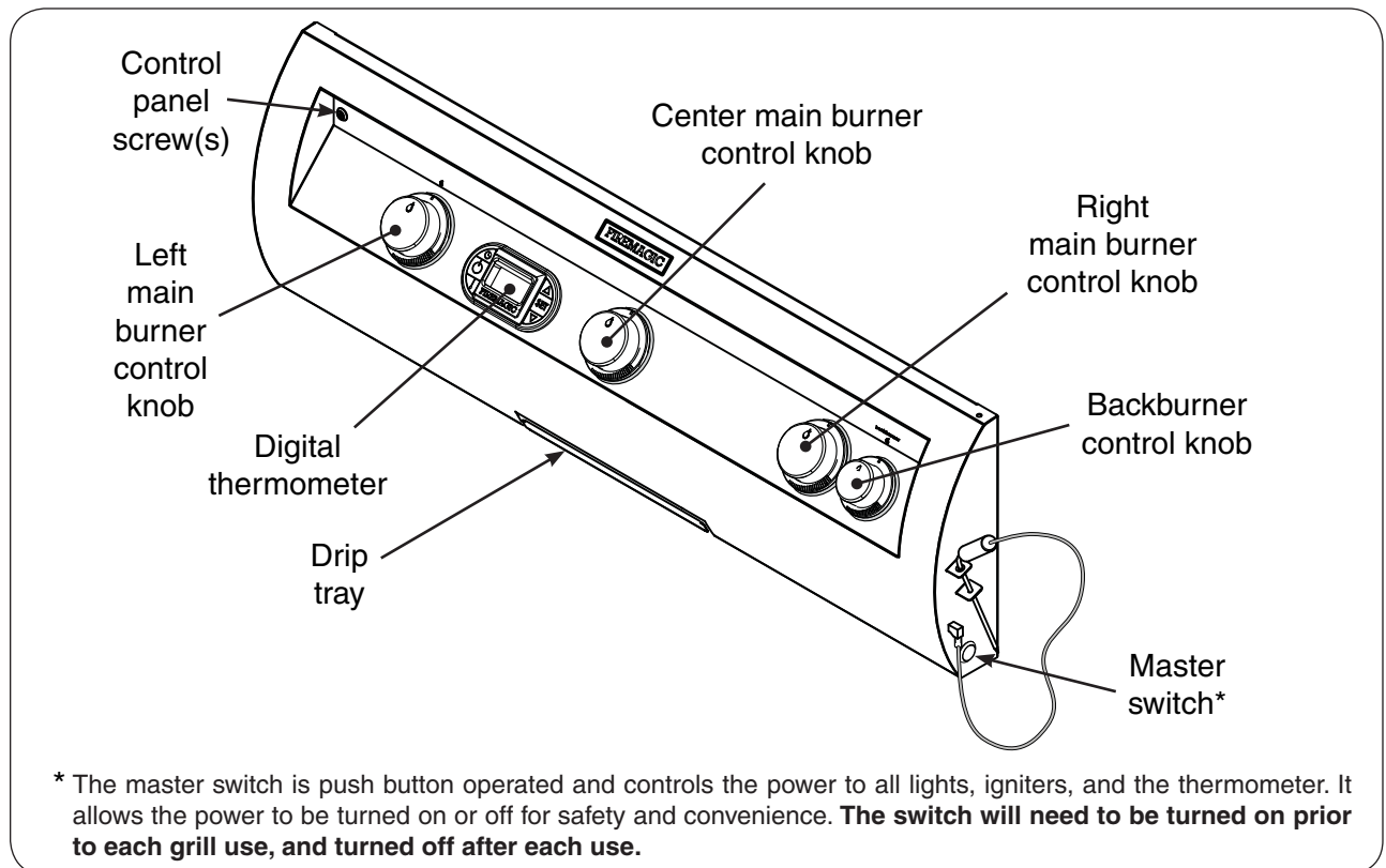
Fig. 22-2 E660i and E790i controls
